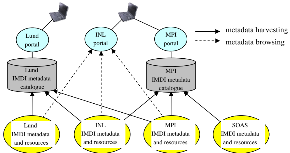
Figure 1 Shared metadata domain. Metadata is harvested from all participants in searchable & browsable catalogue systems by those sites that support it (Lund & MPI). INL supports a browsing only catalogue of the available metadata. SOAS offers metadata for harvesting, but relies on its own catalogue system (not shown).
